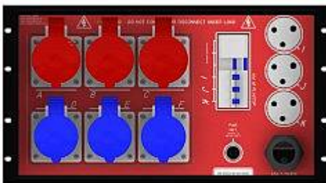
REAR VIEW
