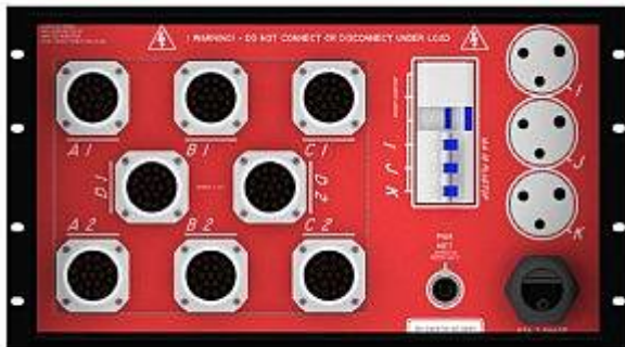
REAR VIEW (8xSOCAPEX VERSION SHOWN)
