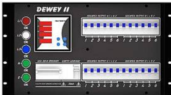
EARTH LEAKAGE VERSION
