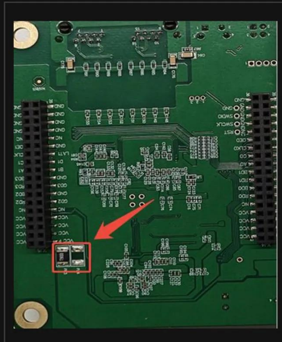
Short circuit protection design
