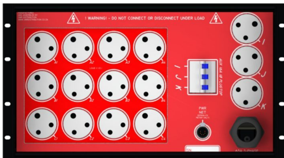
REAR VIEW
