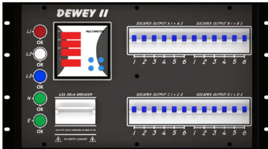
NON - EARTH LEAKAGE VERSION
