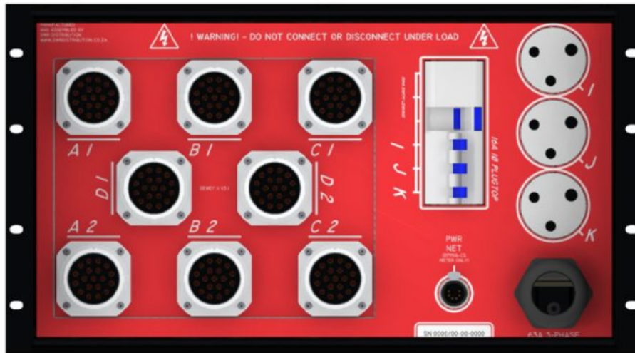
REAR VIEW (8XSOCAPEX VERSION SHOWN)
