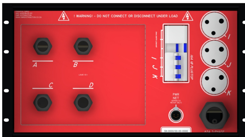
REAR VIEW
